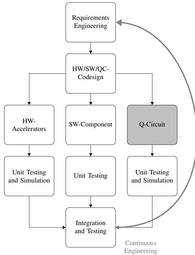
Fig. 2 Quantum Software Development Process
