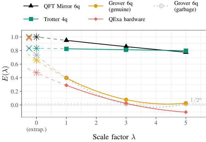
Fig. 2. Richardson extrapolation across signal-retention regimes at \lambda \in \{1, 3, 5\} . Solid: Lagrange polynomial through E(\lambda_k) ; dashed: extrapolation to E(0) (stars); crosses mark E_{\text{ideal}} . Grey dotted: garbage folding on Grover. The Euro-Q-Exa parity signal turns negative at \lambda = 5 (signal destroyed). Horizontal dotted: floor 1/2^6 of the 6-qubit circuits.
