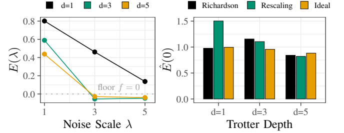
Fig. 1. Richardson extrapolation on Euro-Q-Exa. Left: The amplified parity values E(\lambda) of a 4-qubit QTC collapse to the floor f = 0 as the Trotter depth d grows. Right: At each depth, the Richardson estimate \hat{E}(0) , the rescaling prediction \frac{15}{8} E(\lambda_1) , and E_{\text{ideal}} . Once the signal reaches the floor ( d=3, 5 ), \hat{E}(0) tracks the rescaling and is decoupled from the ideal value; at d=1 , where the signal is retained, it instead recovers the ideal.
